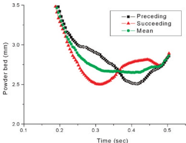
Figure 3. Preceding, succeeding and mean powder bed reduction curves obtained at the maximal compression force of 20 kN and 10 rpm (200 MPa pressure).
