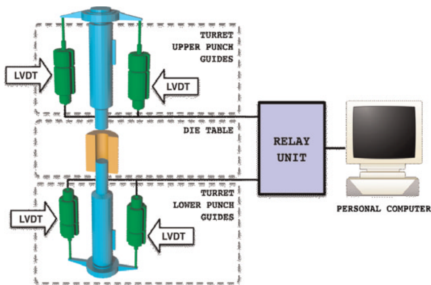
Figure 1. Device for punch displacement control.
